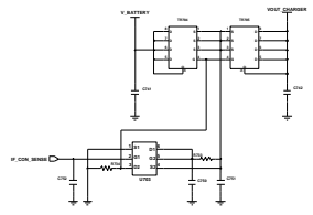
EXT_JIG_POWER_CONTROL
