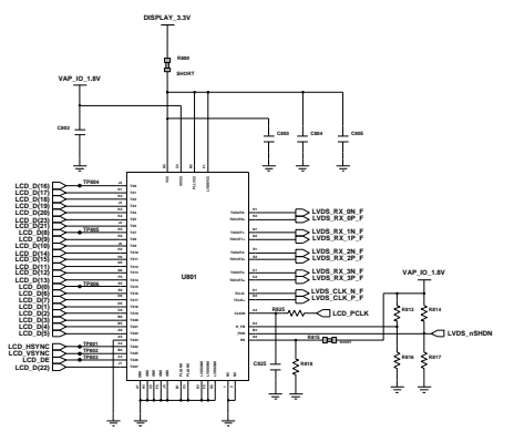
LVDS Transmitter
