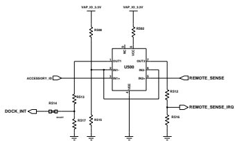
ACCESSORY_INT
