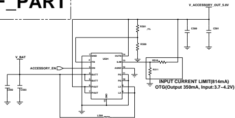
ACCESSORY_PWR
