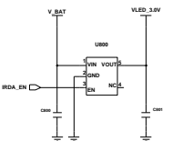
IRDA LDO(option)
