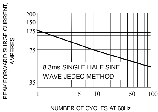
Fig. 5-MAXIMUM NON-REPETITIVE SURGE CURRENT
